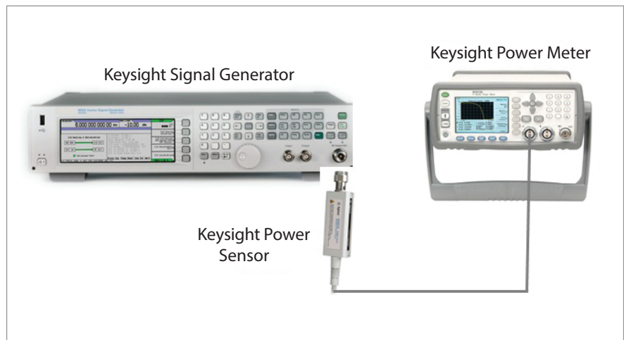
Figure 4. Configuration for obtaining CW and average power measurements
