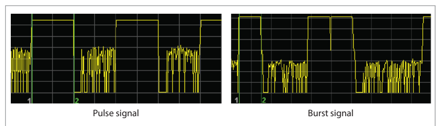
Figure 3. Pulse signal with a constant duty cycle versus burst signal without a constant duty cycle.
